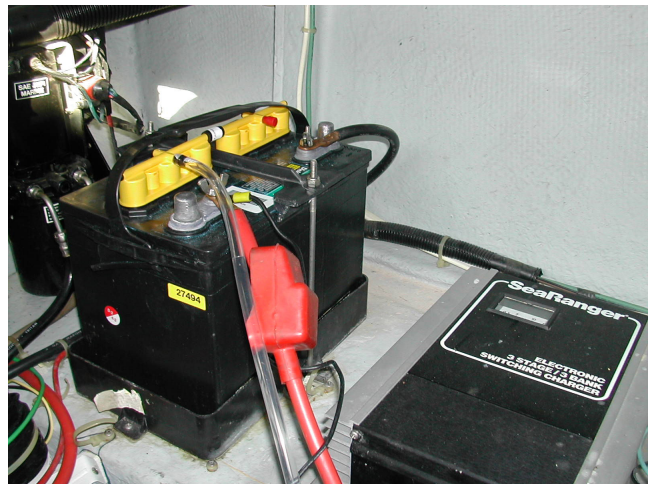
Single Battery to Qwik Connector
